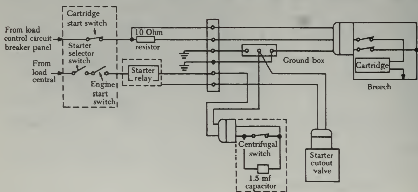
FIGURE 5-22. Cartridge/pneumatic starter electrical schematic.
